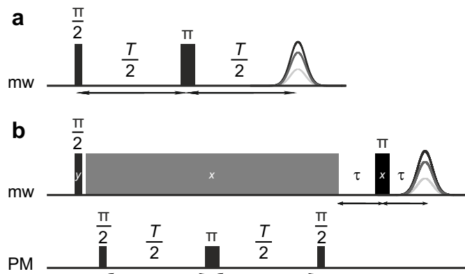
Figure 2. Pulse sequences for measuring bare-spin (a) and dressed-spin (b) decoherence. This spin-lock pulse has constant mw frequency \omega_{mw} and constant amplitude \omega_1 . The phase modulation (PM) pulses have a are cosine-modulated with frequency \omega_T corresponding to \omega_{PM} = \omega_1 matching the amplitude of the mw field of the spin-lock pulse (grey).
