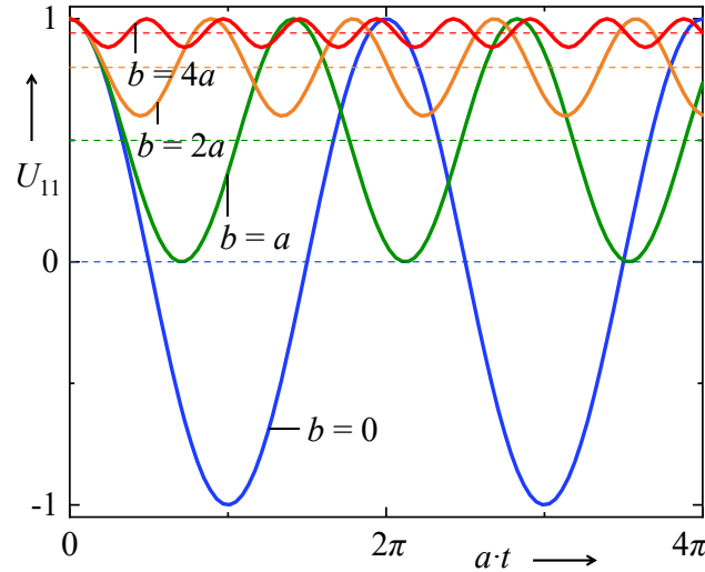
Figure 1. Time evolution of the prefactor of \hat{A} in Eqn. (36) for different ratios b/a . The particular case b = 0 leads to the 2D case; therefore, the corresponding curve is a pure oscillation around zero. With increasing b , the average levels of the related oscillations (dashed horizontal lines) increase whereas the corresponding amplitudes decrease.
