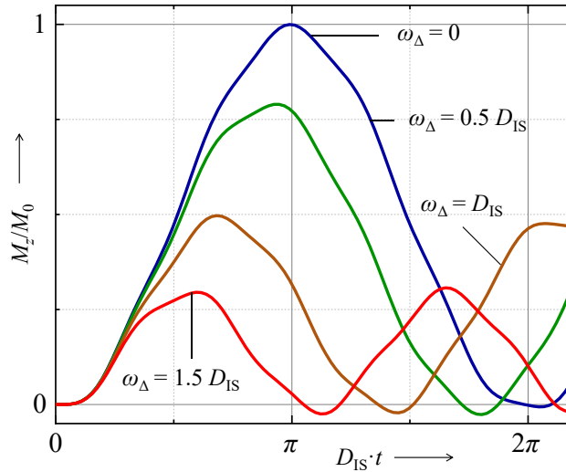
Figure 5. Examples for cross-polarization buildup curves for the I spins in an ensemble of spin pairs I, S corresponding to Eqn. (65) with \omega_{\phi} = 3D_{IS} . The deviation \omega_{\Delta} from the Hartmann-Hahn condition is varied.
