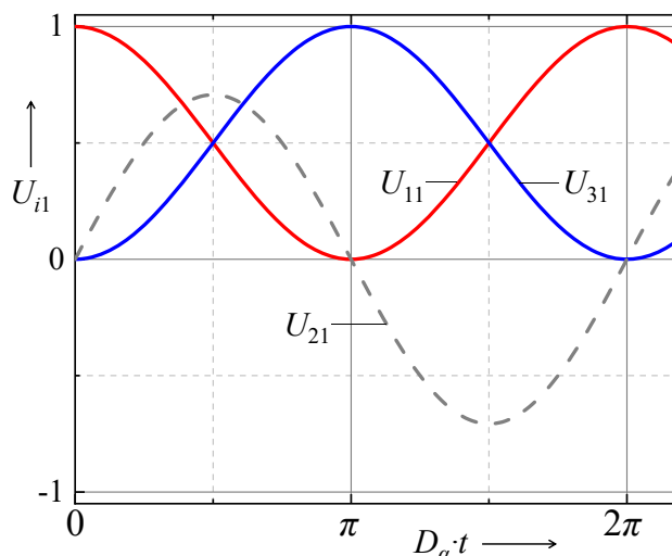
Figure 2. Time evolution of the three prefactors in the propagation rules Eqns. (48) and (49).
