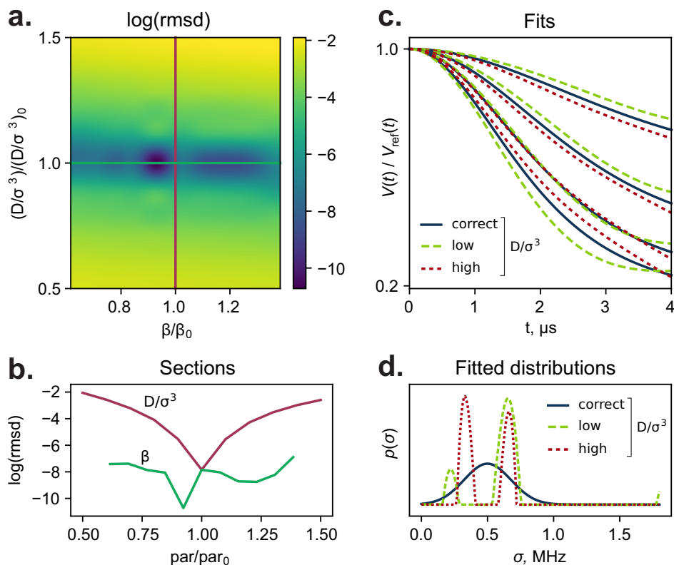
Figure 6. (a) Relaxed scan of D/\sigma^3 and \beta . The axes correspond to the deviations of the scanned parameters from those used for the dataset generation ( (D/\sigma^3)_0 and \beta_0 ). (b) Sections of the rmsd plot in the top left panel where one of the parameters is fixed. (c) Fitting results in time domain with a fixed (D/\sigma^3) of low (green dashed line), optimal (navy solid line) and high value (red dotted line) - respectively, 0.5(D/\sigma^3)_0 , (D/\sigma^3)_0 and 1.5(D/\sigma^3)_0 . (d) Corresponding fitted local proton concentration distributions.
