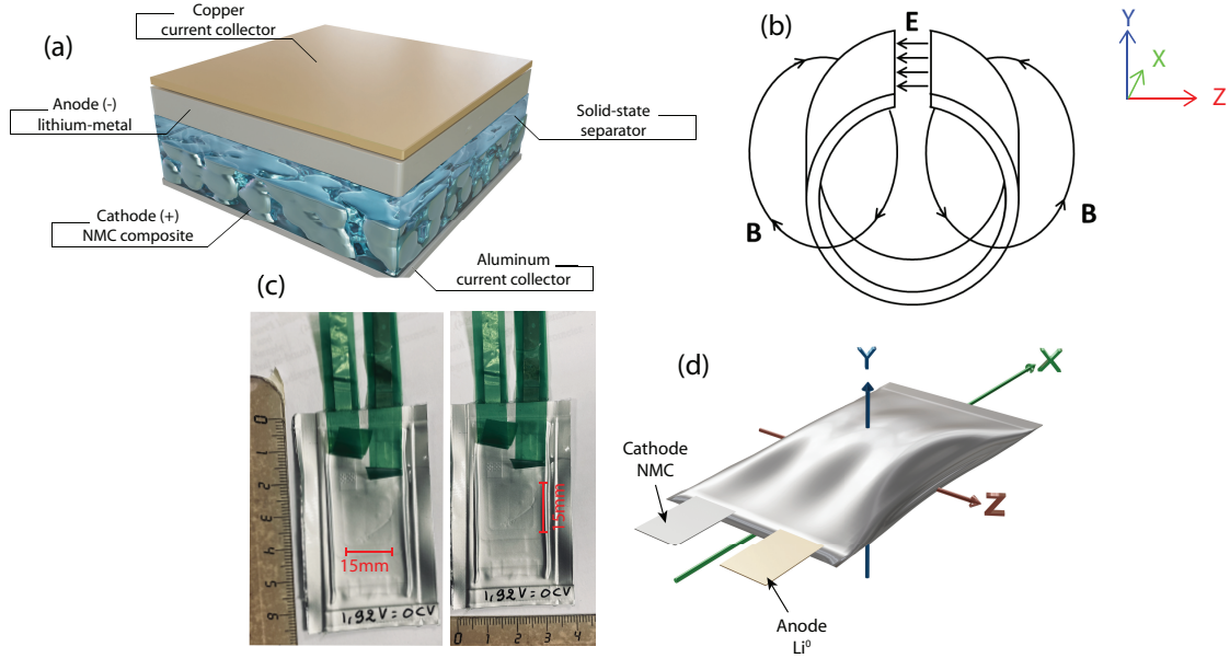
Figure 1. Examples of pouch cells studied in this work. (a) Schematic representation of the stacking used in our solid-state battery NMC||Li 0 . (b) Sketch of a microwave loop-gap cavity used for L-band EPR spectroscopy. The electrical field ( E ) is confined to the capacitive gap whereas the magnetic field ( B ) is confined inside the inductive loop. (c) Digital photos of the NMC||Li 0 pouch cell. (d) Schematic representation of the pouch cell with its orientation inside the microwave loop-gap cavity.
