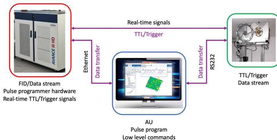
175 Figure 5. Data communication scheme among the workstation PC, NMR console and driving motors.
