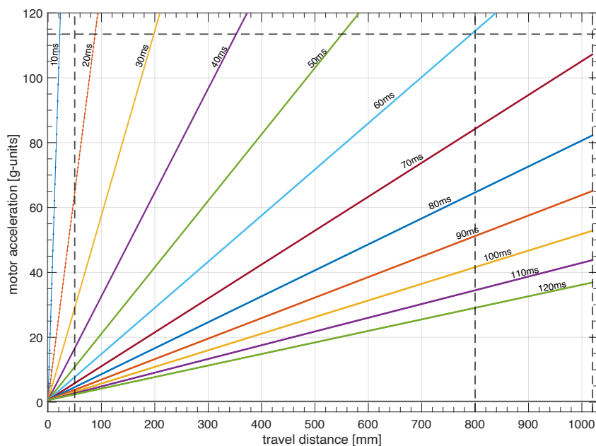
210 Figure 9. Achievable shuttle travel times as function of travel distance and motor acceleration.
