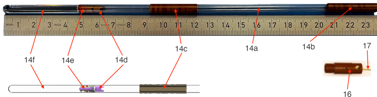
160 Figure 4. Sample container components. 14a – high precision thin wall NMR tube with diameter d = 5 mm and length l = 9 inches, 14b – upper sleeve with thread, 14c – lower sleeve, 14d and 14e – plug elements to limit the sample volume 14f, 16 – end cap with shuttle rope (17) attached.
