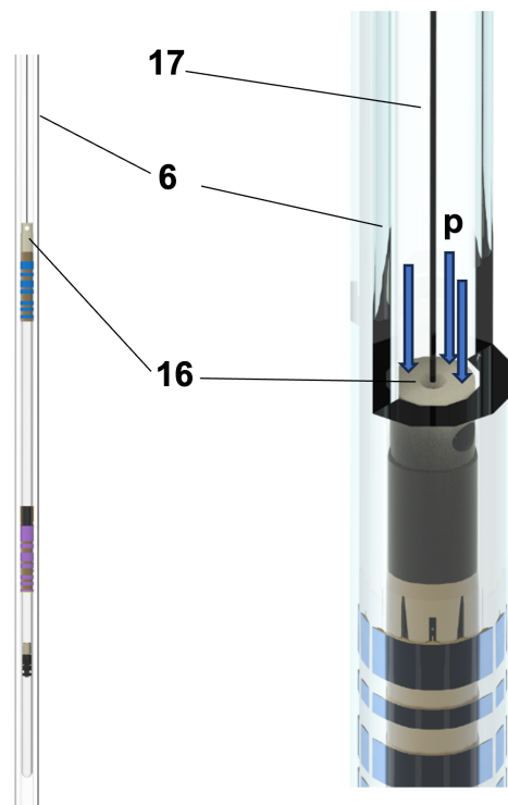
Figure 3. Diagram of sample container in the guidance tube with gas pressure ( p ) applied. 6 – shuttle guiding tube (borosilicate 3.3 glass), 16 – sample container end cap, 17 – shuttle rope (polyethylene).
