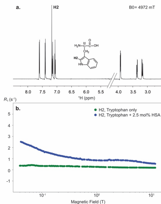
Figure 13. High-resolution proton relaxometry of tryptophan. (a) Structure and one-dimensional proton spectrum of tryptophan at 14.1 T obtained after a transfer to a magnetic field B_{low} = 4.97 T, a relaxation delay T_{rel} = 3 ms and a stabilization delay at high field \tau_{st} = 150 ms. (b) Nuclear magnetic relaxation dispersion profiles for tryptophan proton H2 in the absence (green) and the presence of 2.5% equivalent of human serum albumin (blue).
