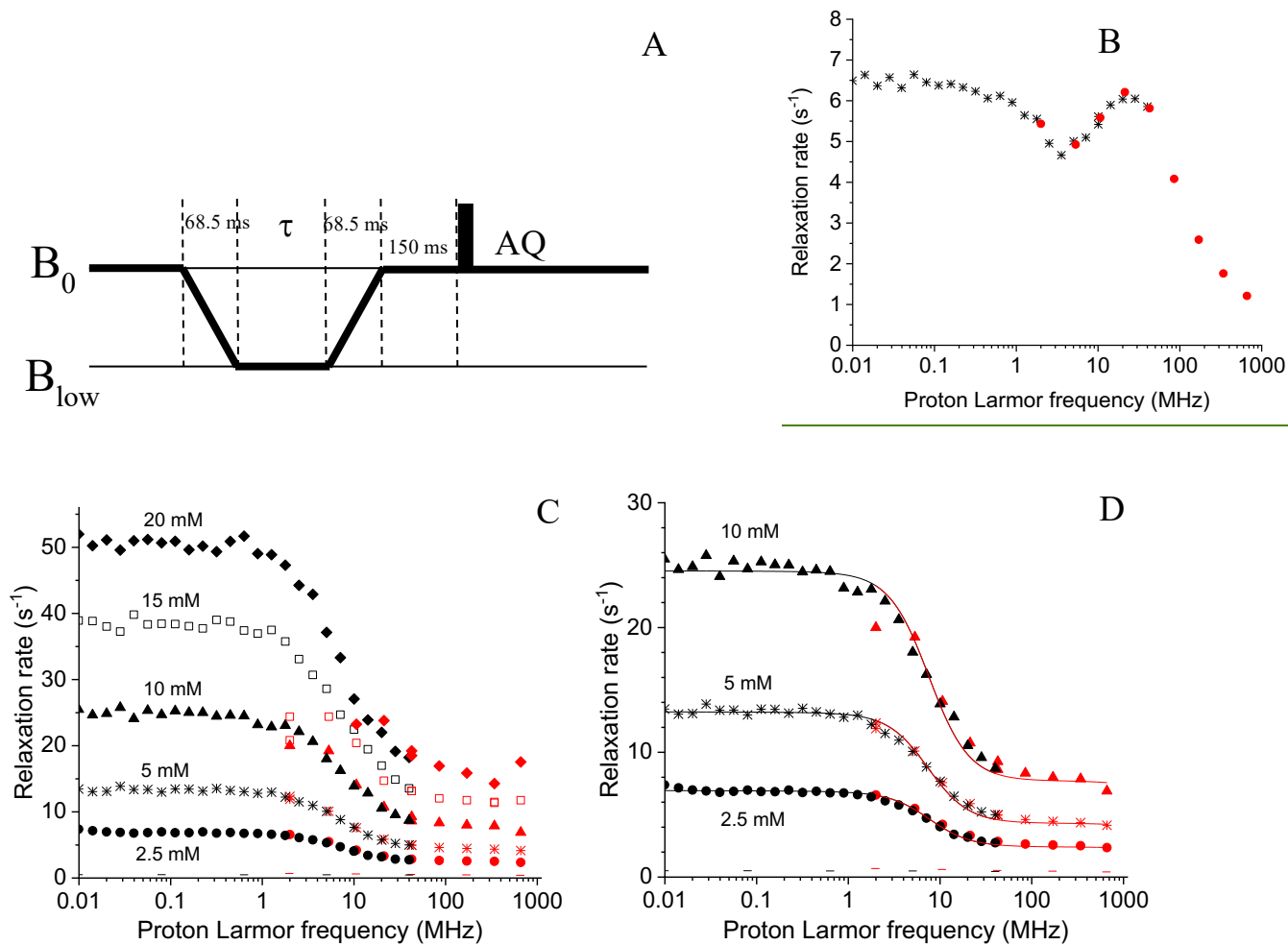
310 Figure 12. (A) Pulse sequence used for the shuttle measurements. The times \tau during which the sample is kept at low fields were set to 16 different values ranging from 0 to 1.75 s. (B) Field dependence of the longitudinal relaxation rates of water protons in a 0.25 315 mM solution of Gd-AIE at 15 °C and (C) in 2.5, 5, 10, 15, and 20 mM solutions of Cu(NO_3)_2 dissolved in a 20 mM HClO_4 solution of 90% H_2O and 10% D_2O , at 15 °C; the – symbols indicate the rates of the buffer alone. Black symbols indicate data collected with the Stellar FFC relaxometer (0.01-40 MHz) and red symbols indicate data collected at the Bruker 700 MHz spectrometer equipped with the shuttle system (2-700 MHz). (D) Best fit profiles of the relaxation rates of water protons in 2.5, 5, and 10 mM solutions of Cu^{2+} aqua ion.
