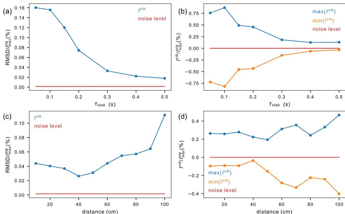
245 Figure 11. Amplitude of vibration artifacts in ^1\text{H} NMR spectra of 99.8% \text{D}_2\text{O} (residual water peak 0.2% \text{H}_2\text{O} ). Vibrations were 250 quantified in the intervals [-200 \text{ Hz}, -20 \text{ Hz}] and [20 \text{ Hz}, 200 \text{ Hz}] around the water peak. The level of the noise (red lines) is given as 255 a comparison. (a-b) Decay of vibration artifacts after shuttle transfer from the furthest distance ( d_{\max} = 1020 \text{ mm} ) at different 260 stabilization times \tau_{st} . (a) root mean square deviations of signal amplitudes normalized by the maximum peak intensity; (b) maximum and minimum intensities of vibration artefacts normalized by the maximum peak intensity. (c-d) Extent of vibrations 150 ms after shuttle landing as a function of the distance of shuttle displacement d . (c) root mean square deviations of amplitudes normalized by the maximum peak intensity; (d) maximum and minimum intensities of vibration artefacts normalized by the maximum peak intensity.
