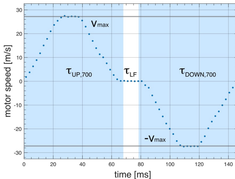
195 Figure 7. Measured shuttle trajectory (motor speed vs. time) for the FSS installed at the 700 MHz NMR spectrometer at CERM in Florence. The relaxation time at the low field position is \tau_{LF} .
