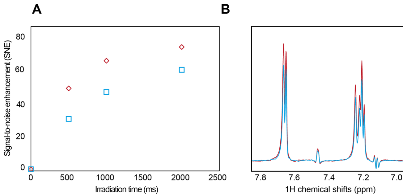
170 Figure 3: A) SNE evolution with illumination time, with illumination from the top (red) and from the bottom (blue). B) signal intensity after 2 seconds of illumination from the top (red) and from the bottom (blue). The sample contained 30 \mu\text{M} tryptophan and 10 \mu\text{M} fluorescein, with oxygen-quenching enzymes, GOCAT, and glucose (see Material and Methods).
