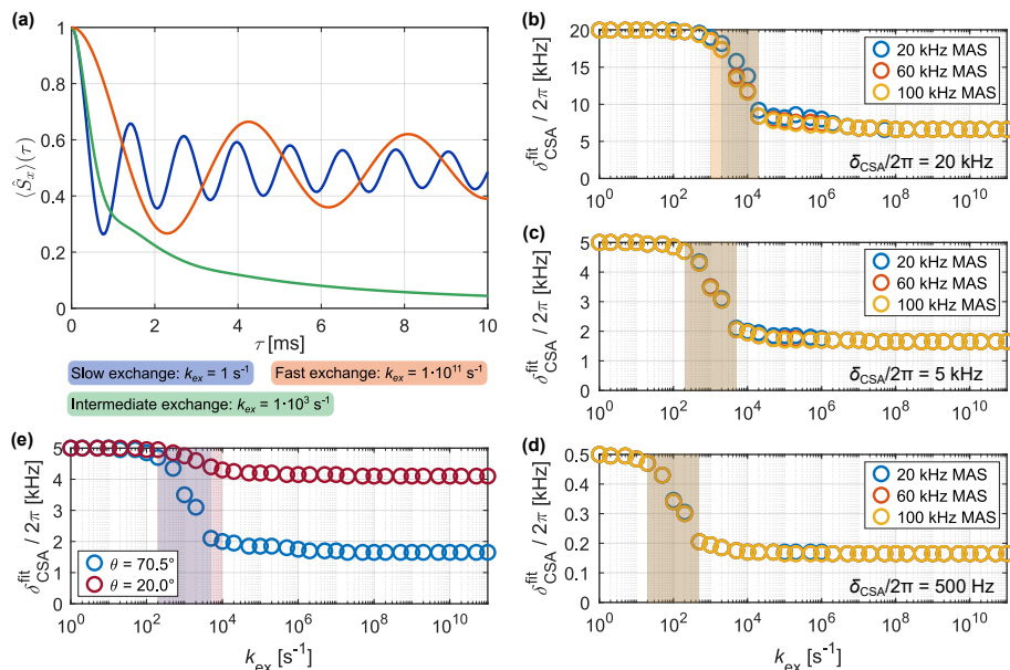
Figure 7. Apparent recoupling behaviour for R181 \bar{1} recoupling of the CSA interaction in the presence of molecular motion. a) Examples of recoupling curves for slow, intermediate and fast exchange (20 kHz MAS, \delta_{CSA}/(2\pi) = 5 \text{ kHz} , \theta = 70.5^\circ ). For fast exchange, a lower frequency oscillation corresponding to the scaled CSA interaction is observed. Motion on an intermediate time scale results in a strong damping of the oscillations and signal decay. b-d) MAS dependence of fit results for different interaction strengths. e) Comparison of fitted apparent \delta_{CSA}^{fit} for different opening angles \theta (20 kHz MAS, \delta_{CSA}/(2\pi) = 5 \text{ kHz} ).
