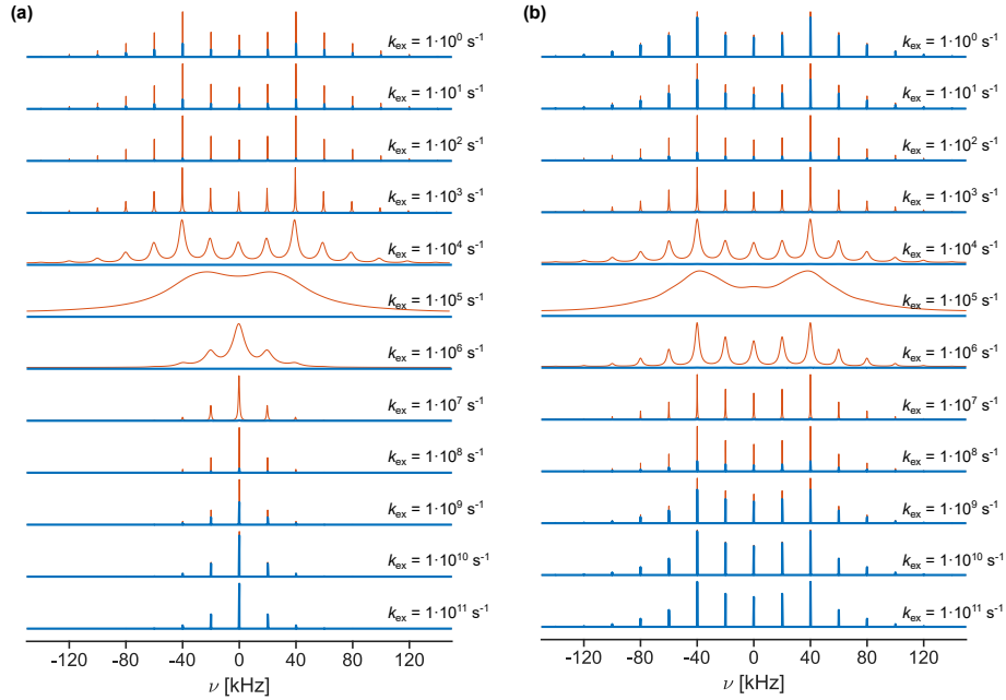
Figure 8. Simulated spectra of ^2\text{H} with \delta_Q/(2\pi) = 80 \text{ kHz} at 20 kHz MAS for different exchange-rate constants for opening angles of \theta = 70.5^\circ (a) and 20^\circ (b) (see Fig. 1a for the geometry of the exchange process). The intensity of spectra shown as thick blue lines was normalized to the maximum intensity observed for all exchange-rate constants while spectra shown as thin red lines were normalized to their respective maximum intensity. All spectra were processed with 10 Hz exponential line broadening. For exchange-rate constants around 1 \cdot 10^5 \text{ s}^{-1} , the sideband manifold is broadened beyond detection due to rapid relaxation.
