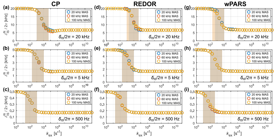
Figure 3. Fitted apparent anisotropy of the dipolar-coupling tensor \delta_{\text{IS}}^{\text{fit}} for CP (a-c), REDOR (d-f) and wPARS (g-i) for different MAS frequencies (20, 60 and 100 kHz) and dipolar-coupling strengths ( \delta_{\text{IS}}/(2\pi) = 20, 5 and 0.5 \text{ kHz} ). The underlying molecular motion was modeled using a three-site jump process with an opening angle of \theta = 70.5^\circ (order parameter S_{\text{IS}} = -1/3 ), which corresponds to the case of a sp^3 -hybridised carbon site. The rf field strengths used for the recoupling are summarized in Table S2 in the SI. For slow exchange, the full dipolar coupling is retained, while the scaled interaction is observed for fast exchange. In the intermediate exchange regime, a smooth transition from the full to the scaled coupling is observed (shaded area, defined as the region where the difference between two consecutive fitted \delta_{\text{IS}}^{\text{fit}} exceeds 6 % of the difference between the full and scaled \delta_{\text{IS}} used in the simulations). The position of this transition region depends on the coupling strength and occurs at slower motions for smaller couplings. The MAS frequency only has a marginal effect on the location of the intermediate regime.
