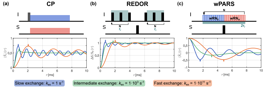
Figure 2. Examples of simulated dipolar recoupling curves for (a) CP, (b) REDOR, and (c) wPARS for slow, intermediate and fast exchange (20 kHz MAS, \delta_{\text{IS}}/(2\pi) = 5 \text{ kHz} , \theta = 70.5^\circ ). In the intermediate exchange regime, a damping of the oscillations is observed while fast exchange simply leads to a scaling of the dipolar coupling and, thus, a reduction of the oscillation frequency. The apparent \delta_{\text{IS}} is determined by \chi^2 -fitting a set of reference simulations with different heteronuclear dipolar couplings without exchange to the initial build-up of the recoupling curve (up to the first local extremum, position indicated by arrows).
