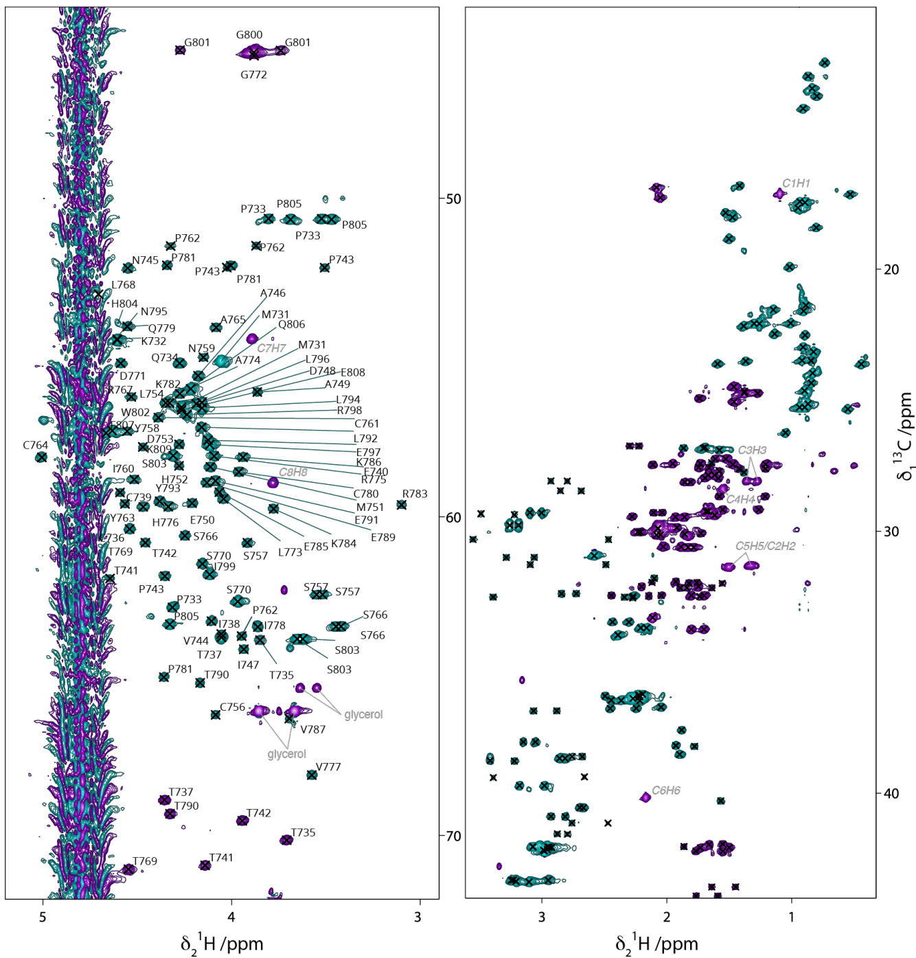
Figure 3: ^{13}\text{C} -HSQC spectrum of ^{13}\text{C} - ^{15}\text{N} Gn cyto . (A) \text{C}\alpha/\text{H}\alpha region with assignments shown on the spectrum. (B) Side-chain region, with crosses indicating assigned peaks. For assignments see BMRB submission. Few impurities are observed, which correspond to desthiobiotin (labeled in italic grey) and glycerol (labeled in grey).
