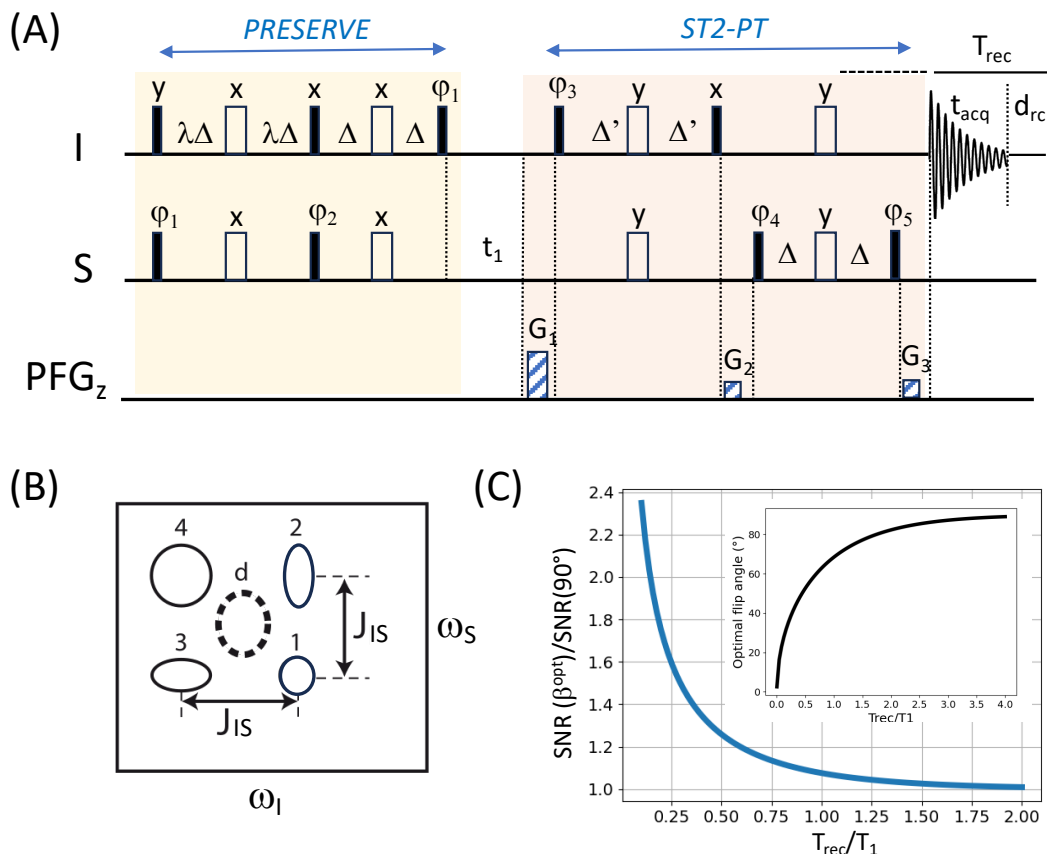
Figure 1. PRESERVE-TROSY experiment for recording heteronuclear 2D I-S correlation spectra. (A) The pulse sequence comprises the PRESERVE, t 1 , and ST2-PT building blocks. Filled and open pulse symbols correspond to 90° and 180° rf pulses, respectively. The appropriate single-transition spin-states are selected by adjusting the pulse phases φ 3 and φ 5 , as well as the gradients G 1 , G 2 , and G 3 . Echo/anti-echo quadrature detection in t 1 is achieved by the pulsed field gradients G 1 , G 2 , G 3 with (G 1 -G 2 )/(G 3 -G 2 ) = ± γ I /γ S , and inverting phases φ 3 and φ 5 for the anti-echo component. Phase inversion of the whole PRESERVE sequence by 180° together with the receiver phase improves the line shapes of the detected NMR signals. In addition, axial peak suppression can be realized by inverting phases φ 4 and φ 5 together with the receiver phase. The heteronuclear transfer delay is set to Δ = 1/(4J IS ), while Δ' should be chosen slightly shorter in order to reduce the intensity of residual anti-TROSY components. (Schulte-Herbrüggen and Sørensen, 2000) Small flip angle (β) excitation of I and S spin polarization is achieved by tuning the scaling factor λ to λ = β/90°. (B) Multiplet structure of NMR peaks detected in a scalar coupled I-S spin system, corresponding to the individual single-transition states of the I- and S-spins. This multiplet pattern can be reduced to a single peak using either heteronuclear spin decoupling (HSQC: peak d) or spin-state selection (TROSY: either one of the 4 peaks). (C) Numerical simulation of the expected sensitivity gain if an optimal flip angle is chosen instead of the common 90° nutation, as a function of the T rec /T 1 ratio. The plot in the insert shows the computed optimal flip angle as a function of the T rec /T 1 ratio according to equation (1). These simulations neglect spin relaxation and pulse imperfections.
