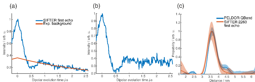
Figure C 14: (a) 4 pulse-SIFTER of first echo in 4 pulse-SIFTER experiment with a pulse length ratio of 2-2-6-3 and sweep directions of up-down-down-down averaged over the whole nitroxide spectrum (blue) and exponential background fitted by DeerAnalysis (orange). Since the first echo only appears if third pulse is included, there is no SIDRE equivalent for the first echo. (b) Formfactor obtained by division of blue trace of (a) by orange background in (a). (c) Distance distributions obtained by Tikhonov regularisation in DeerAnalysis of PELDOR trace recorded at Q-band (blue) and of SIFTER formfactor in (b) (orange).
