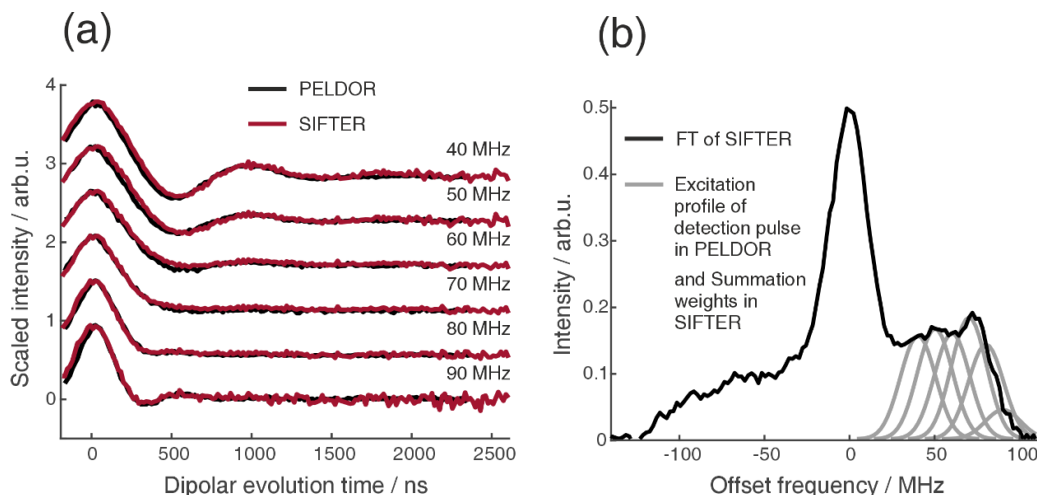
Figure 9: Comparison of 2D-SIFTER and orientation selective PELDOR time traces of a doubly \zeta m-labelled RNA duplex recorded at X-band frequencies. (a) Orientation selective PELDOR traces with detection pulses applied at offsets 40 – 90 MHz from the position of the pump pulse (black) and slices of the 2D-SIFTER experiment weighted by the Gaussian-shaped pulse excitation profiles of the detection pulses used in the PELDOR experiment (red). The SIFTER traces were first divided by the corresponding SIDRE traces and afterwards by an exponential; for the PELDOR traces a typical background correction was applied. Afterwards, all traces were scaled to the same modulation depth. (b) FT of the SIFTER echo at \tau_2 - \tau_1 = 0 in black and excitation profiles of the detection pulses used in the PELDOR experiments shown in light grey for the different offset positions. The excitation profiles correspond to the summation weighting for generation of the SIFTER slices shown in (a).
