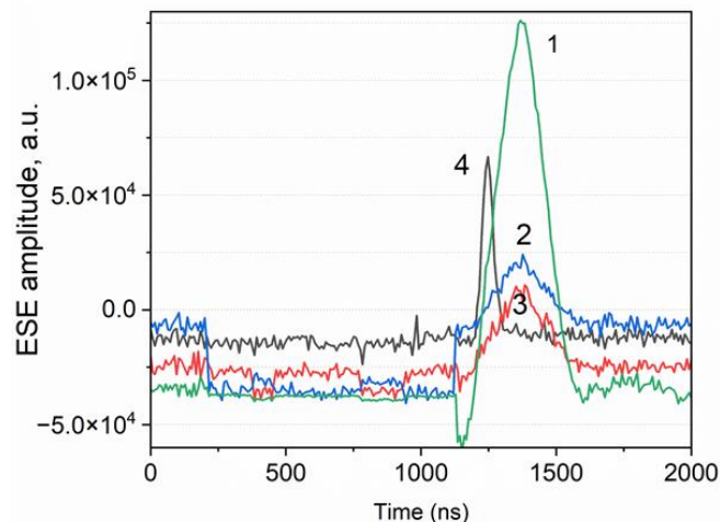
145 Figure 5: Hahn echo with BDPA:PS in a 0.5 mm ID quartz capillary measured at 294 K in: 1 – bimodal probehead in transmission mode with LNA (Patt=18 dB; \pi/2 -pulses = 80 ns; \pi -pulses = 160 ns); 2 - bimodal probehead without LNA in reflection mode; 3 - EN 5107D2 probehead (Patt= 24 dB; \pi/2 -pulses = 80 ns; \pi -pulses = 160 ns); 4 - EN 5107D2 probehead (Patt= 0 dB; \pi/2 -pulses = 6 ns; \pi -pulses = 12 ns). All traces were recorded with single shot per point, and with 400 ns delay between the pulses.
