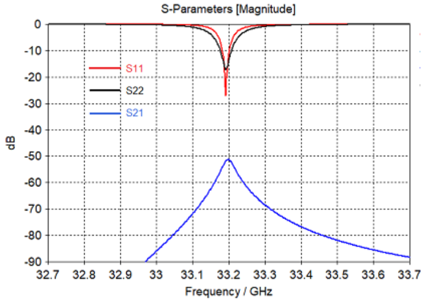
105 Figure 3: Microwave properties of TE103 bimodal c simulated by CST Suite: S11 (red) - input port reflection coefficient; S22 (black) 110 - output port reflection coefficient; S21 (blue) - transmission coefficient that indicates output-to-input isolation between input and output ports.
