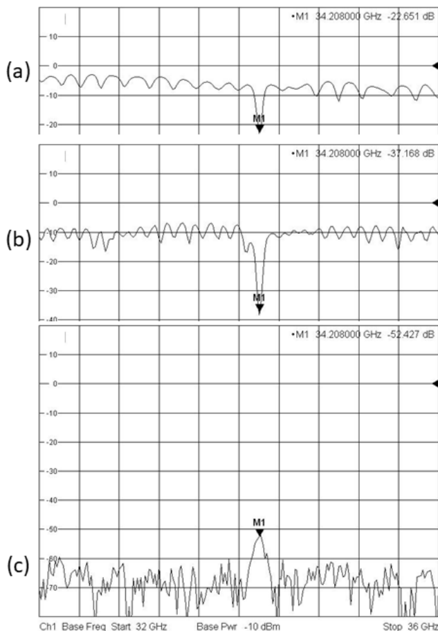
Figure 4: a) Return loss of the probehead input for switch position 1-3; b) Return loss of the cavity output when the network analyzer is connected to the output position as indicated in Fig. 1; c) Input-to-output isolation of the probehead without the LNA. On the left: input and output modes are tuned to the same frequency of 34.208 GHz. On the right: output mode was detuned to 34.342 GHz (134 MHz above the input mode).
