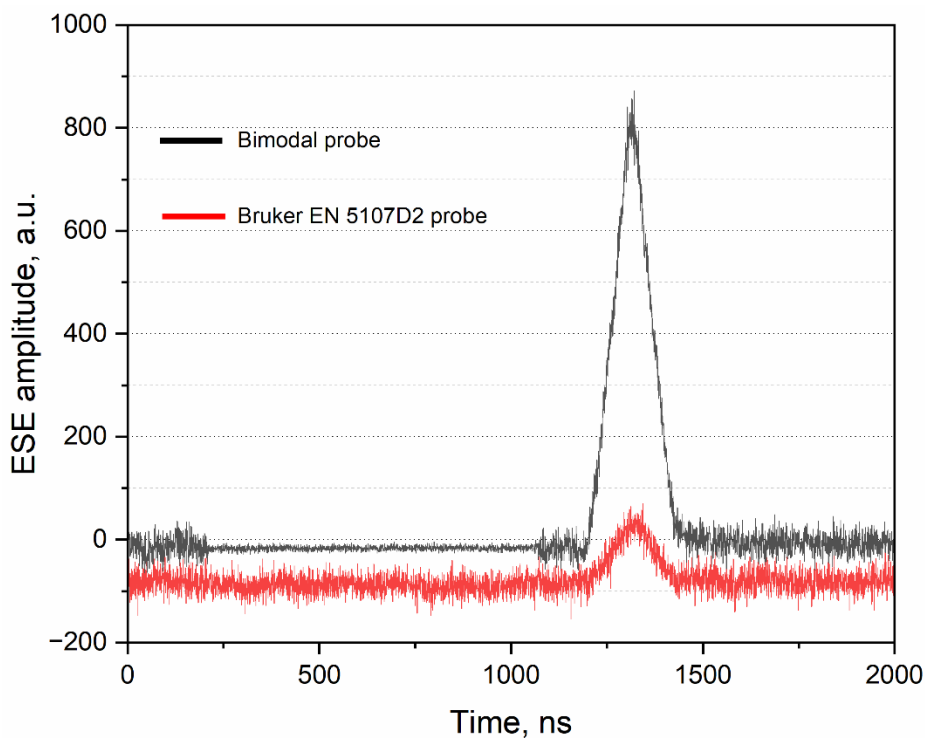
Figure 6: Spin echo with 0.1 mM OXO TEMPO in toluene measured at 80 K by a typical Hahn echo experiment in: black – a 2.8 mm OD sample tube inside the bimodal probehead (Patt=15 dB; \pi/2 -pulses = 50 ns; \pi -pulses = 100 ns); red – a 1.6 mm OD sample tube inside the EN 5107D2 probehead (Patt= 22 dB; \pi/2 -pulses = 50 ns; \pi -pulses = 100 ns). All traces were recorded with single shot per point, and with 400 ns delay between the pulses. Video gain is 6 dB. In the region between 200 ns and 1100 ns where the spectrometer protection gate is ON the noise for the bimodal cavity trace (black one) is lower because it is reduced proportionally due to normalization step of the large signal produced by the LNA which has 30 dB gain.
