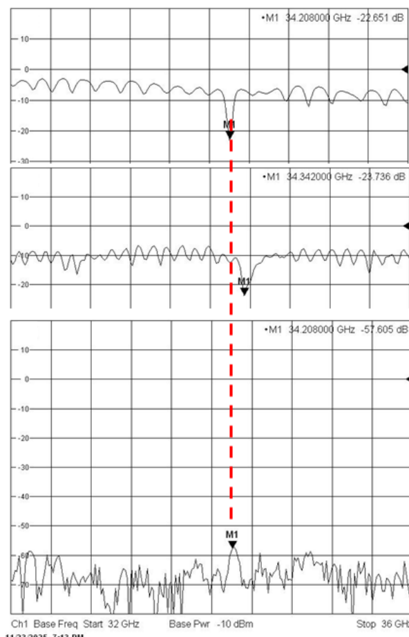
Figure 4: a) Return loss of the probehead input for switch position 1-3; b) Return loss of the cavity output when the network analyzer is connected to the output position as indicated in Fig. 1; c) Input-to-output isolation of the probehead without the LNA. On the left: input and output modes are tuned to the same frequency of 34.208 GHz. On the right: output mode was detuned to 34.342 GHz (134 MHz above the input mode).
