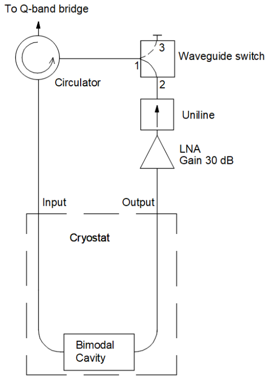
65 Figure 1: Block-diagram of the Q-band EPR probehead. The waveguide switch is shown in the position 1-2 for transmission mode operation. Reflection mode is available when the switch is in the position 1-3.
