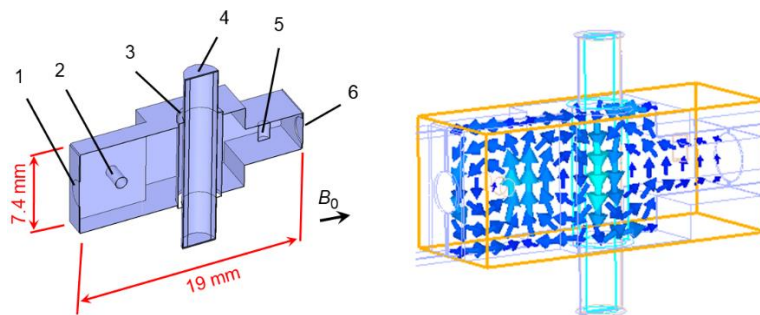
Figure 2: Bimodal TE103 cavity. On the left: 1 – input port with coupling iris 2.2 mm diameter, 2 – quartz rod 1 mm diameter for input mode frequency tuning; 3 – teflon tube 4mm OD / 3 mm ID for resonator protection against impurities; 4 – quartz sample tube 2.8 mm OD; 5 – quartz rod 1.5 mm diameter for output mode frequency tuning; 6 – output port with coupling iris 3 mm diameter. Input and output ports have similar 7.4 \times 3.7 mm cross-sections. All other dimensions of the structure are included in a 3D model in SI (Supplementary Information). On the right: microwave B_1 field distribution along the cavity is demonstrating the decoupling between output and input ports (simulated by CST Suite).
