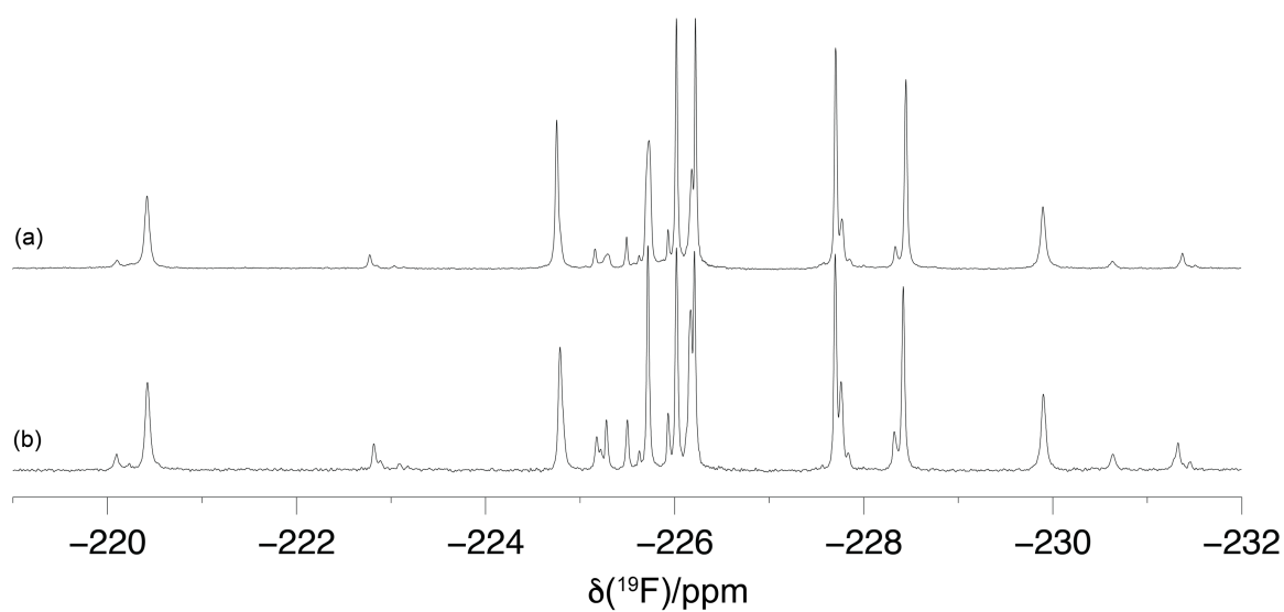
Figure. 1D {}^{19}\text{F} -NMR spectra of two different preparations of GB1-d. (a) 3 mM solution in 50 mM HEPES buffer, pH 7.5, 100 mM NaCl. (b) 1 mM solution in 20 mM MES buffer, pH 6.5, 100 mM NaCl. The {}^{19}\text{F} chemical shifts are insensitive to the solution conditions.
