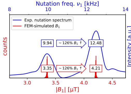
Figure 4. Dual x -axis plot superimposing the experimental nutation spectrum interpolated by a cubic spline (blue) and the FEM-simulated B_1 distribution (red). The nutation spectrum was recorded using rectangular pulses of varying pulse length at a constant pulse power (see Sec. 2.2). The FEM-simulated B_1 distribution was obtained as a histogram of the B_1 magnitudes at all the finite volume elements of the cavities. The smaller \nu_1 and B_1 values correspond to the PEEK cavity while the larger \nu_1 and B_1 values correspond to the copper cavity. The relative difference between the \nu_1 maxima (25.6 %) is in good alignment with the relative B_1 increase predicted by the FEM simulation (25.7 %).
