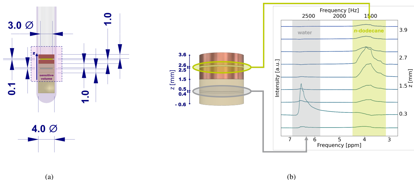
Figure 1. Sectional side view of experimental setup inside a shortened standard 5 mm NMR tube with cell dimensions given in mm (a) and 3D illustration of setup with a spatially-encoded chemical shift imaging of \text{H}_2\text{O} and n -dodecane in between the double coins (b). The cavities each have a diameter of 3 mm and a height of 0.1 mm. The coins each have a diameter of 4 mm and a height of 1 mm. The NMR-sensitive volume for homogeneous excitation is marked by a pink hue and extends \pm 4 mm in z -direction from the center of the model setup. The spatial position of the liquids can be differentiated on a scale of about half a mm.
