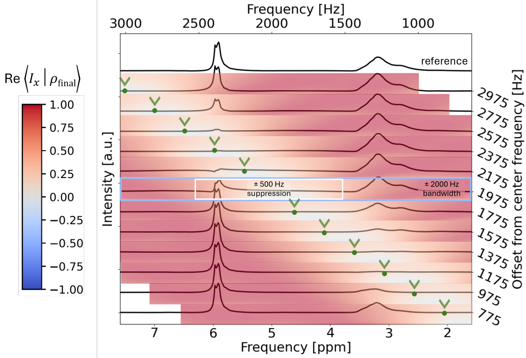
Figure 3. ^1\text{H} spectra recorded utilizing a \nu_0 -selective suppression pulse with a selective suppression range of 2.5 ppm ( \pm 500 Hz), 2 ms duration, and a total frequency range of 4000 Hz applied at different \Delta\nu_0 . The top spectrum depicts the reference ^1\text{H} spectrum recorded using a hard pulse. Hereby, the resonance at approx. 3 ppm is assigned to n -dodecane and the resonance at approx. 6 ppm to \text{H}_2\text{O} . The spectra recorded with QOC pulses are overlaid with colour gradients representing the theoretical x -magnetization \text{Re}\langle I_x | \rho_{\text{final}} \rangle , normalized to a range [-1, 1] , after applying the QOC pulse at each particular \Delta\nu_0 . Selective suppression is achieved for the on-resonance pulses with \Delta\nu_0 = 2375 Hz for \text{H}_2\text{O} and \Delta\nu_0 = 1375 Hz for n -dodecane.
