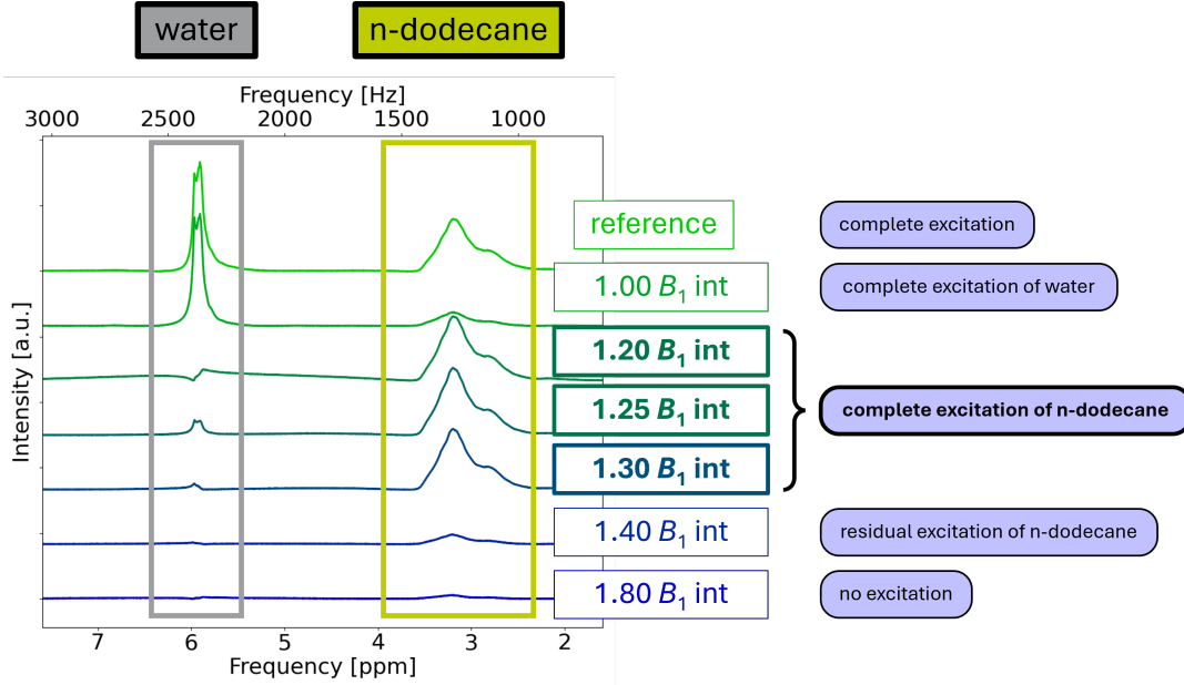
Figure 5. ^1\text{H} spectra recorded utilizing \nu_1 -selective excitation pulses with a selective excitation range of \Gamma_{B_1} \pm 0.1 , 1 ms duration, and a total frequency range of 2000 Hz. Hereby the resonance at approx. 3 ppm (framed in bright green) is assigned to n -dodecane and the resonance at approx. 6 ppm (framed in grey) to \text{H}_2\text{O} . The top spectrum depicts the reference ^1\text{H} spectrum recorded using a hard pulse. Below, spectra utilizing selective QOC pulses, optimized for increasing \Gamma_{B_1} , are displayed. Selective excitation of n -dodecane is achieved for 1.20 \leq \Gamma_{B_1} \leq 1.30 , which matches the B_1 amplification of the cavity in between copper.
