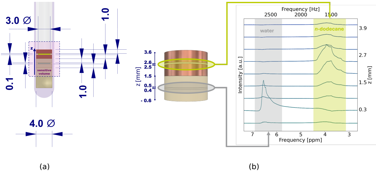
Figure 1. Sectional side view of experimental setup inside a shortened standard 5 mm NMR tube with cell dimensions given in mm (a) and 3D illustration of setup with a spatially-encoded chemical shift imaging of H 2 O and n -dodecane in between the double coins (b). The cavities each have a diameter of 3 mm and a height of 0.1 mm. The coins each have a diameter of 4 mm and a height of 1 mm. The NMR-sensitive volume for homogeneous excitation is marked by a pink hue and extends \pm 4 mm in z -direction from the center of the model setup. The spatial position of the liquids can be differentiated on a scale of about half a mm.
