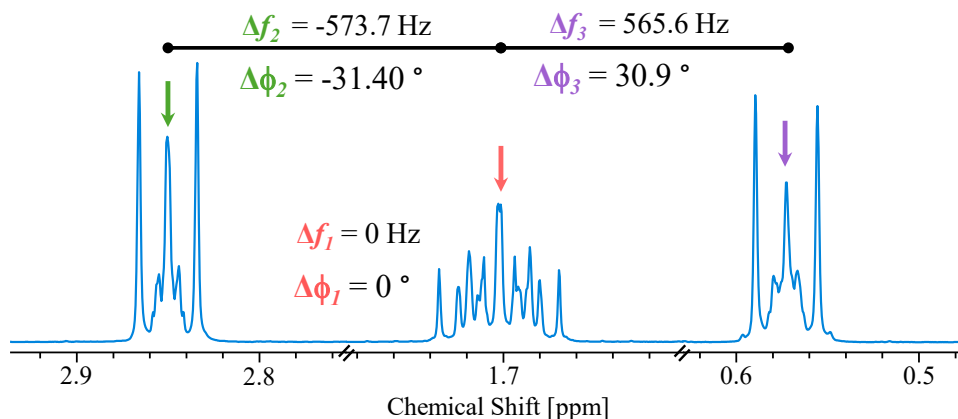
85 Figure 2: One-dimensional (1D) ^1\text{H} spectrum showing peaks corresponding to the three \text{CH}_2 groups of 200 mM sodium trimethylsilylpropanesulfonate (DSS) in 100 mM phosphate buffer solution (PBS, pH 7.2) in \text{D}_2\text{O} at 11.7 T (500 MHz for ^1\text{H} ) showing the phase incrementation required for trichromatic SSL ( M = 3 ) with \Delta t = 152 \mu\text{s} , the carrier frequency being set on the central peak (red arrow). The green and purple arrows designate the positions irradiated using phase incrementation which are calculated with Eq (1) to coincide with the central lines of the high- and low-frequency multiplets. 90
