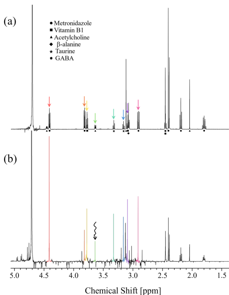
Figure 9: Line-narrowing and decoupling by octa-chromatic SSL applied to a mixture of six small molecules: metronidazole, vitamin B1, acetylcholine, \beta -alanine, taurine and GABA, all at 10 mM concentrations in 100 mM PBS (pH 7.2) in D_2O . (a) Conventional 1D spectrum. (b) Lines narrowed and decoupled spectrum obtained by octa-chromatic SSL as described in the text. The 8 coloured arrows in (a) correspond to the irradiation frequencies of the pulses chosen to spin-lock 8 selected proton signals. The colour-coded peaks in (b) show the corresponding irradiated peaks after line-narrowing and decoupling by octa-chromatic SSL. The wavy arrow indicates the RF carrier frequency. To increase the number of data point across the peaks, a Lorentzian line broadening of 0.3 Hz was applied so that each peak is represented by 5 points. The SNR are boosted by factors between 20 and 27. Both spectra were recorded with 16 k points and 2 scans.
