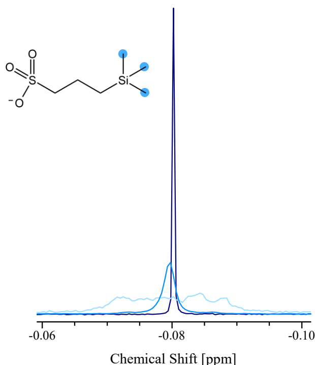
Figure 3: Line-narrowing by monochromatic SSL applied to the three equivalent CH 3 groups (blue circles) of 200 μM DSS in D 2 O. Blue line: Conventional 1D spectrum with a line-width \Delta\nu = 1 Hz. Light blue line (scaled x2): Broadened to a line-width of about 10 Hz by deliberately miss-setting a shim current. Dark blue line: Line narrowed to \Delta\nu = 0.23 Hz by monochromatic SSL applied to the broadened light blue resonance, as described in the text. All spectra were obtained with 64 k points and 2 scans.
